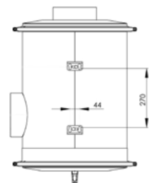
Wall Mounting
