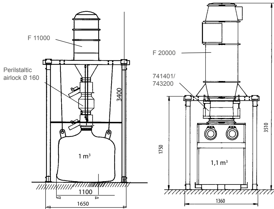
F 20000 with widening chassis and discharge into a 1.1 m 3 container.
